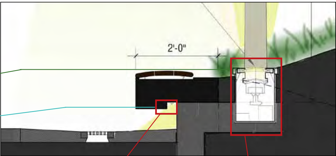
Detail Section
